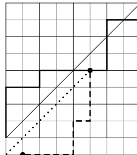
Figure 5: Reflection of a prefix with respect to y = x - 1 .
